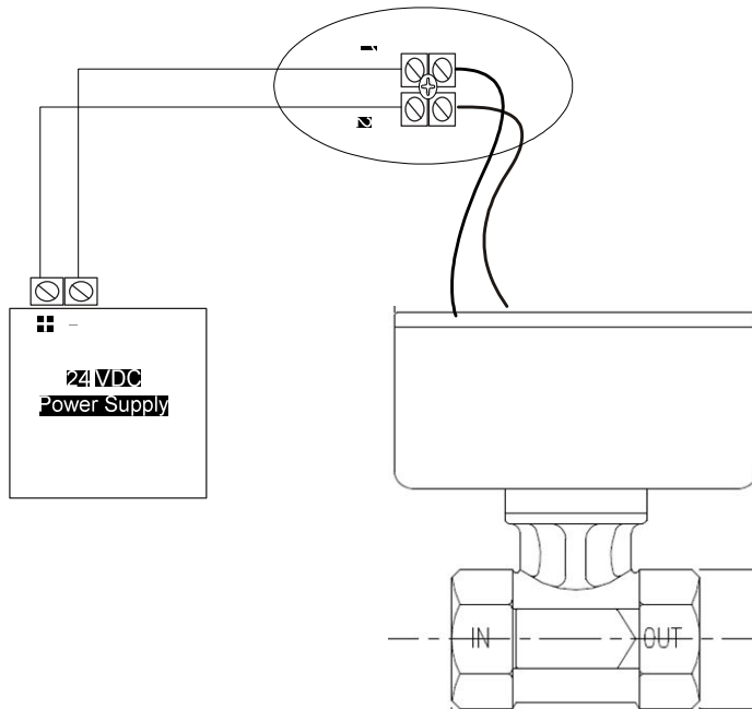
W3-1 Option Wiring
