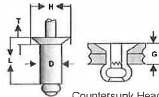
Countersunk Head 120°
